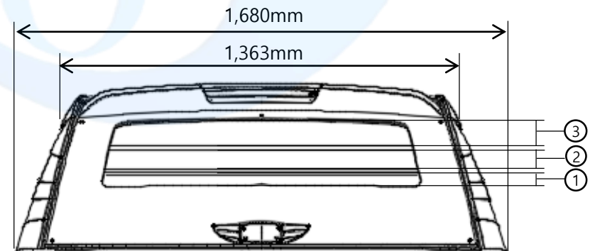
HIGH TOP L10 도어-①100mm, ②100mm, ③100mm
