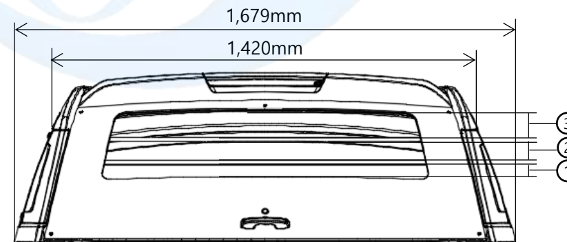
HIGH TOP G10L 도어-①100mm, ②100mm, ③100mm
